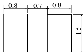
Recommended Solder Pattern
